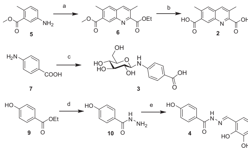
Scheme 1. Synthesis of compounds 2–4 . Reagents and conditions: (a) Yb(OTf) 3 , ethyl glyoxylate, propanal, CHCl 3 , O 2 , 90 °C, 16 h, 20%. (b) NaOH, MeOH/H 2 O, 70 °C, 12 h, 35%. (c) D-Glucose 8 , EtOH, rt, 12 h, 50%. (d) Hydrazine, EtOH, reflux, 48 h, 50%. (e) 2,3-Dihydroxybenzaldehyde, EtOH, AcOH, reflux, 24 h, 66%.
