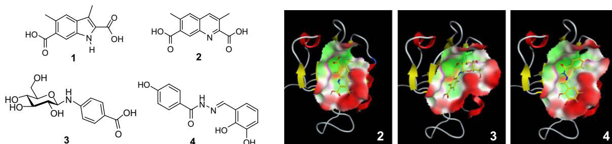
Figure 3. Indole 1 and the best docked poses for the top ranked molecules: quinoline 2 , glycosylamine 3 , N-acyl hydrazone 4 .
