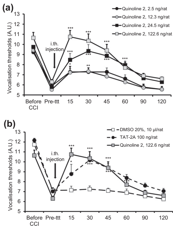
Figure 5. Anti-hyperalgesic effect of quinoline 2 in CCI rats ( n = 8–18 rats per dose). (a) CCI rats were i.t. injected with the indicated dose of quinoline 2 . (b) CCI rats were i.t. injected with either quinoline 2 (122.6 ng/rat), or TAT-2A (100 ng/rat) or vehicle (20% DMSO 10 µl/rat). The vocalisation thresholds to paw pressure (Randall and Selitto test 22 ) were measured up to 120 min after injection. * P < 0.05 , ** P < 0.01 , *** P < 0.001 compared with values measured before drug or vehicle injection (Pre-treatment values).
