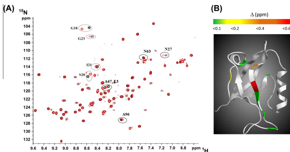
Figure 4. (A) Overlay plot of 1 H– 15 N HSQC spectra of free PSD-95 PDZ2 (black) and in the presence of compound 2 (red) (protein/ligand 1:10). (B) Chemical shift perturbation (CSP) of PSD-95 PDZ2 resulting from compound 2 . \Delta (ppm) = \sqrt{(\text{DH})^2 + (0.15\text{DN})^2} . I.e., the nitrogen difference should be scaled by 0.15.
