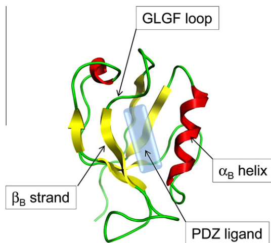
Figure 1. 3D representation of PSD-95 PDZ1 (PDB 2KA9). Helices in red, strands in yellow, loops in green.
